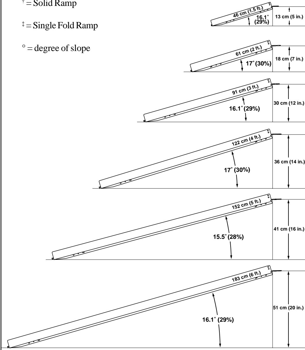
Figure 1. Maximum Ramp Height and Incline Angle
